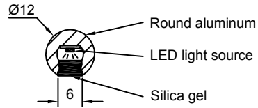
Sectional view
